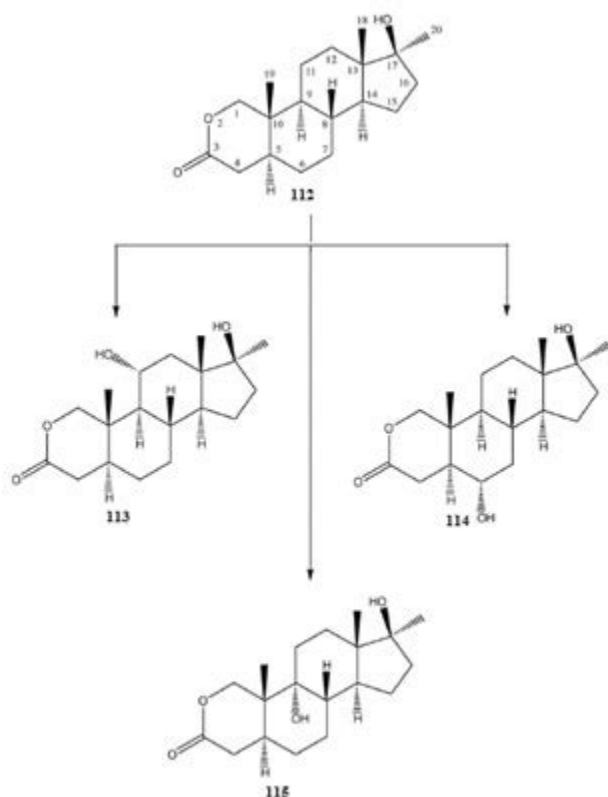
Fig. 23: Biotransformation of oxandrolone (112) with Rhizopus stolonifer .
