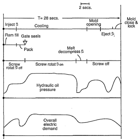
Representative timing diagram, with pressure and electrical power demand profiles for a 28-s machine cycle.
