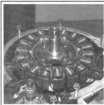
Fig. 23b ...the stator coil windings mounted under the flywheel
