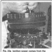
Fig. 23a Ignition power comes from the magneto comprised of the flywheel-mounted magnets and...
