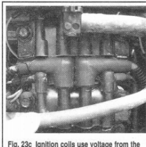
Fig. 23c Ignition coils use voltage from the EHM to induct high voltage that fires the spark plugs
