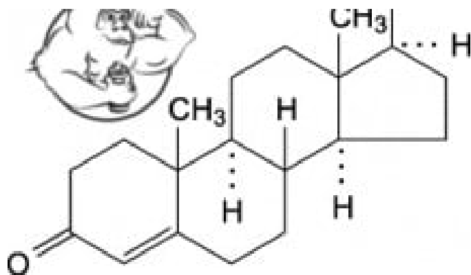
Testosterone
