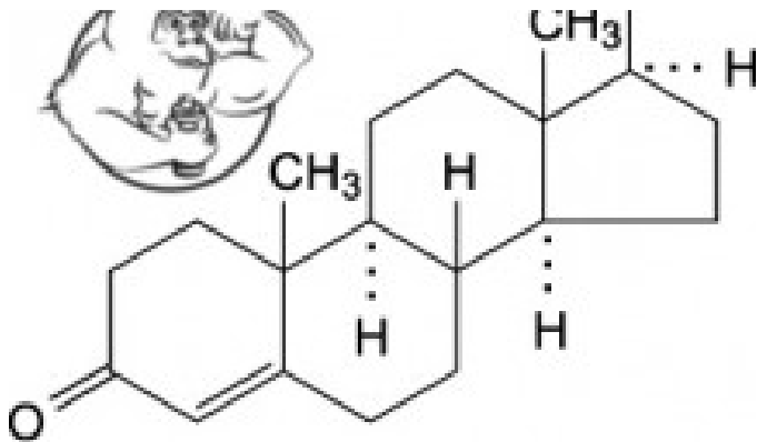
Testosterone
