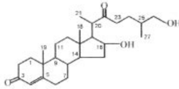
SN-2 (C 27 H 42 O 4 )
