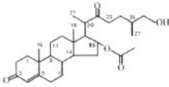
SN-1 (C 29 H 44 O 5 )
