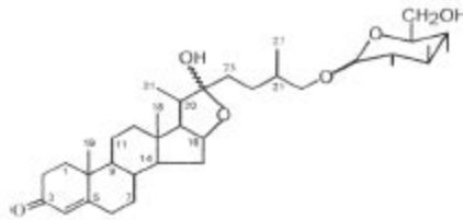
SN-4 (C 33 H 52 O 9 )
