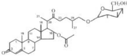
SN-3 (C 35 H 54 O 10 )
