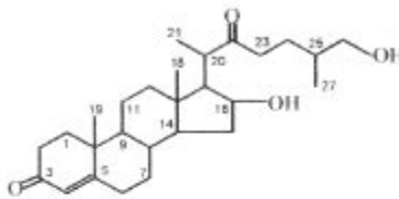
SN-2 (C 27 H 42 O 4 )
